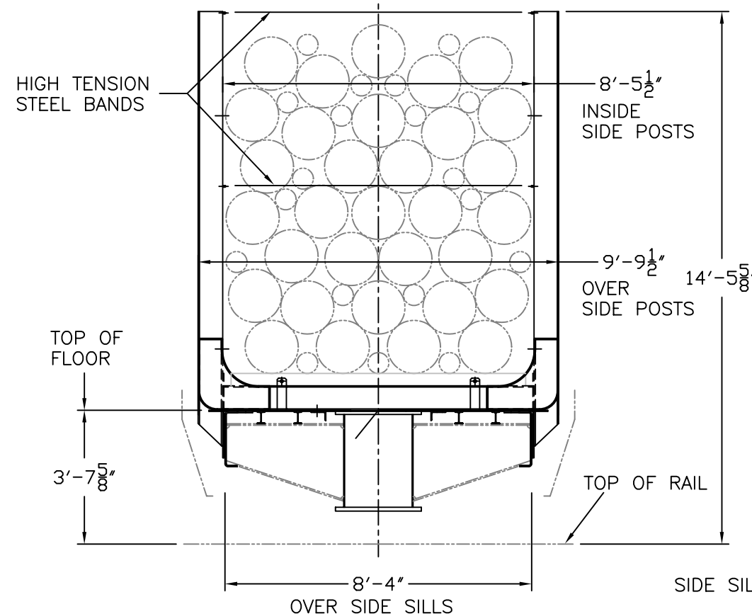
SECTION THROUGH LOADED CAR
